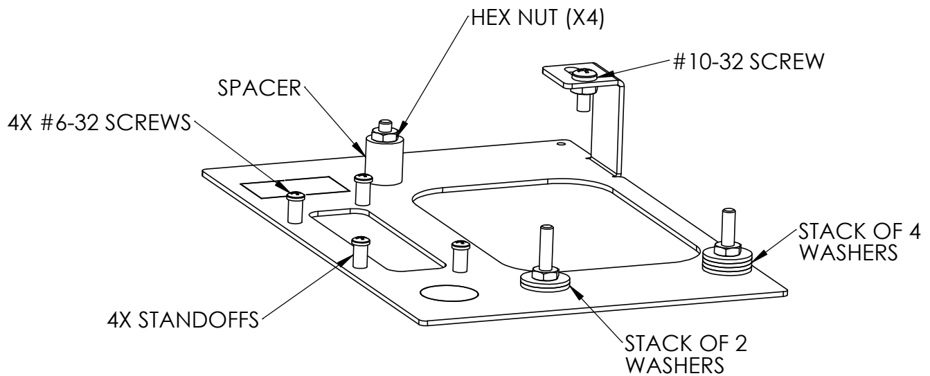
Fig 7 - Rotary Gear Shifter Faceplate with Hardware
